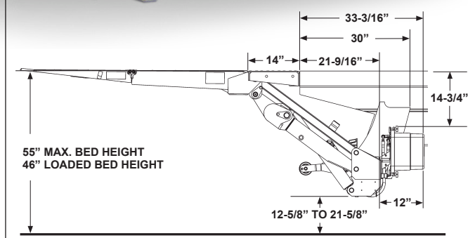
GPT Lift Dimensions and Mounting Requirements
